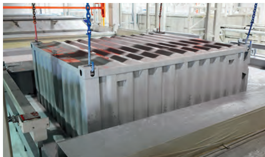
Cathodic electro dip paint grounding
