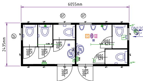
Ladies/Gents Toilet Block 20'
