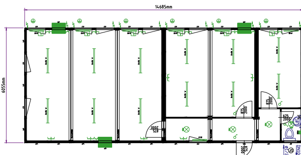
Portable and sanitary cabin 6 units
