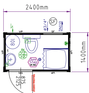
WC shower cabin 8'
